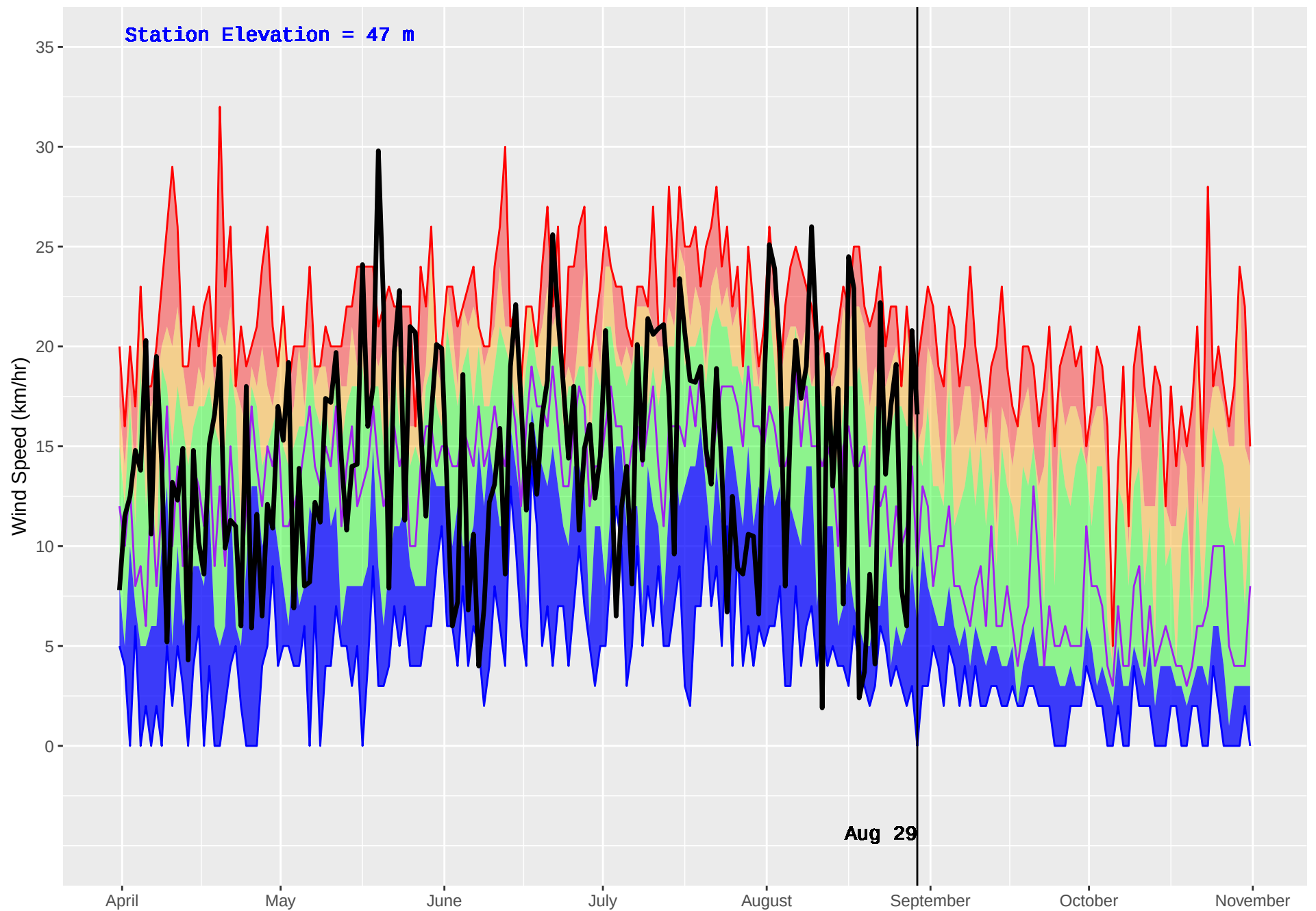
HAGENSborg 2 (904) : Historical (2005–2016) and Current (2018) Daily Wind Speed
