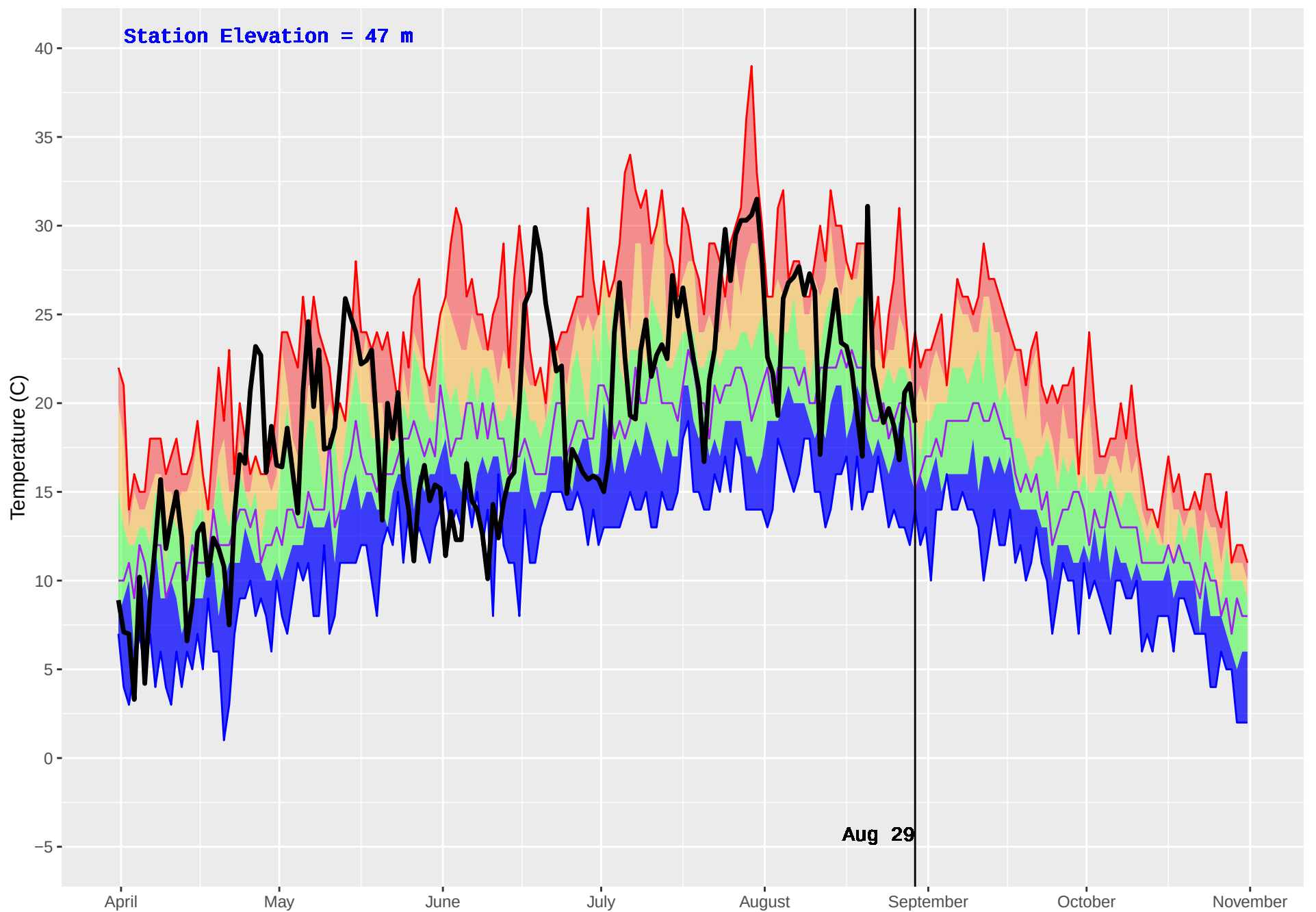
HAGENSborg 2 (904) : Historical (2005–2016) and Current (2018) Daily Temperature
